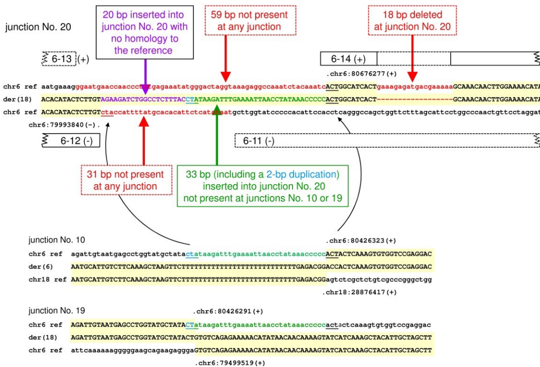
Figure 3. Nucleotide sequence of the highly complex junction No. 20. The sequences present at the junction are in capital letters and highlighted in yellow. Joined segments 612 original neighboring segments 6-11 and 6-13 are indicated by dashed rectangles. Deleted, moved, duplicated and inserted DNA stretches are shown in red, green, blue and violet, respectively. Sequences labeled "ref" and "der" show the reference sequences and sequences of the derivative chromosomes, respectively. Junctions No. 10 and 19 which both lack the 33 bp templated segment (inserted into junction No. 20) are shown for comparison. The microhomologies flanking the 33 bp segment and its insertion site are underlined and connected by curved arrows.
