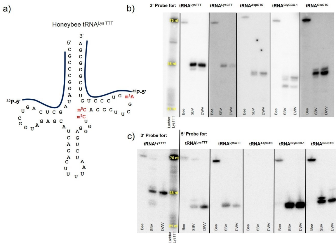
Figure 3. Detection of tRNAs in RNA isolated from Honeybee, SBV and DWV. a) Structure of Honeybee tRNA Lys T TT . b) Northern blot analysis of isolated RNA and in vitro prepared RNA ladder with 32 P labeled probes for 3' end of tRNA Lys T TT , tRNA Lys C TT , tRNA Asp G TC , tRNA Gly G CC-1 and tRNA Glu C TC . c) Northern blot analysis of isolated RNA and in vitro prepared RNA ladder with 32 P labeled probes for 3' end of tRNA Lys T TT and 5' end of tRNA Lys T TT , tRNA Lys C TT , tRNA Asp G TC , tRNA Gly G CC-1 and tRNA Glu C TC . (Experiments were performed in triplicate).
