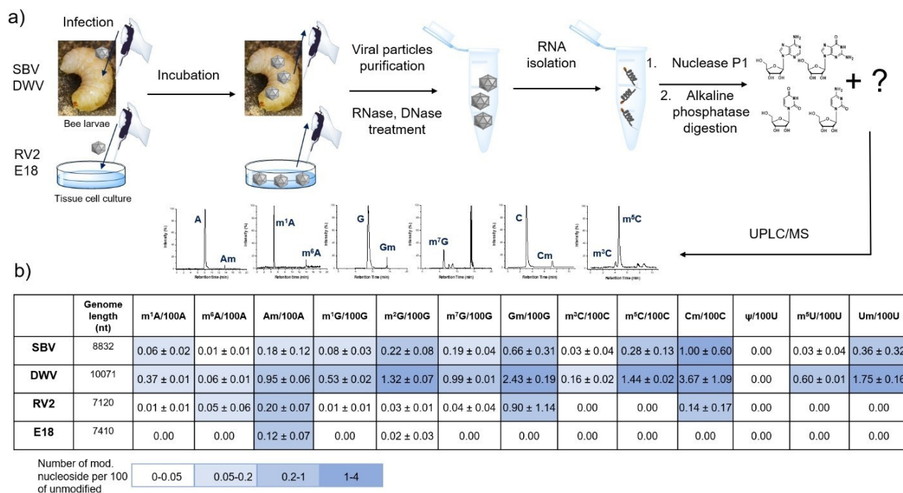
Figure 1. LC-MS analysis of RNA isolated from virions of insects I flaviviruses (SBV, DWV) and human Picornaviruses (RV2, E18). a) Scheme of workflow. b) Table with detected modified nucleosides per 100 unmodified for every virus. The shade of blue indicates the amount of detected methylated nucleoside.
