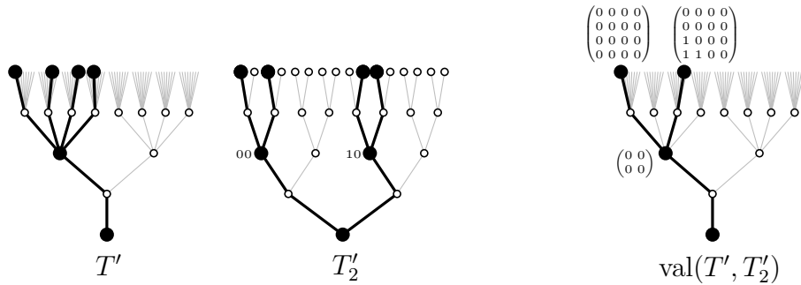
Figure 1.8: An example of a valuation tree
