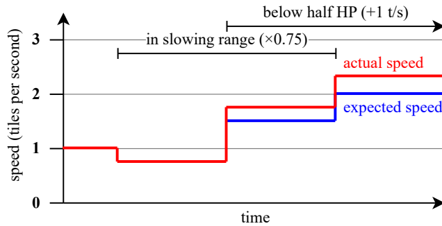
Figure 3.28 Possible discrepancy when multiple effects change an attacker’s speed.
