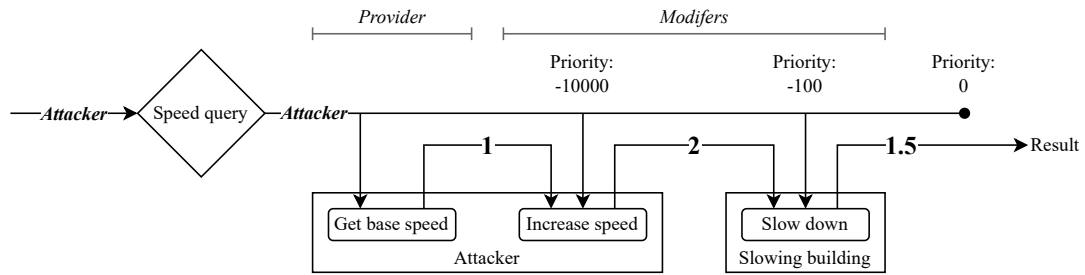
Figure 3.30 Modifiable query for determining attacker speed.
