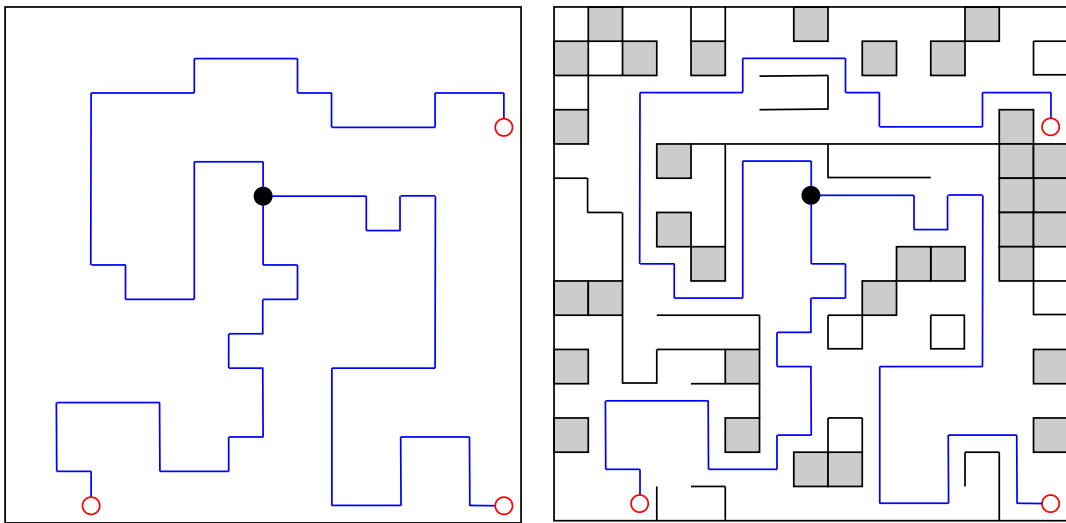
Figure 3.6 Blocked edges and tiles after generating the terrain and obstacles.
