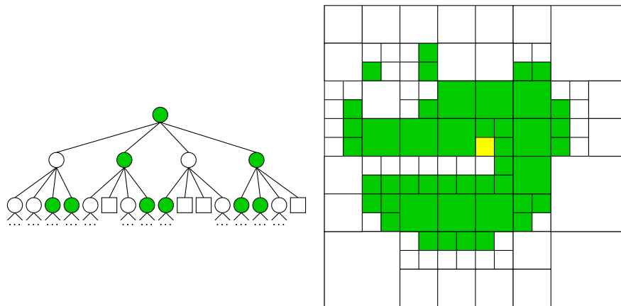
Figure 3.26 Compressed quadtree range representation.
