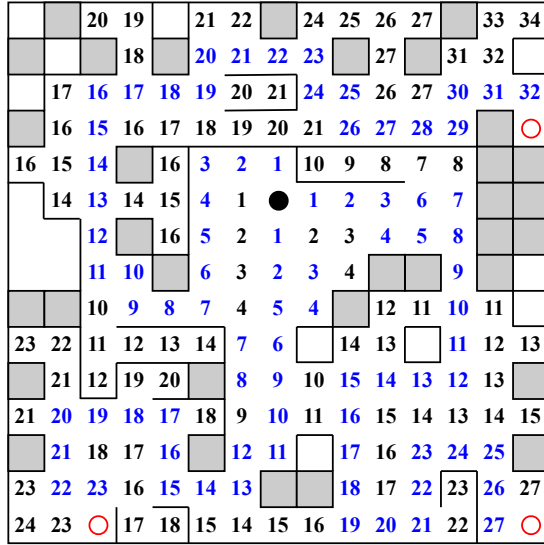
Figure 3.8 Calculated minimum distances.
