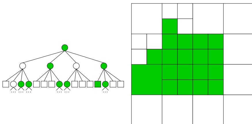
Figure 3.24 Quadtree range representation after expanding 11 nodes.
