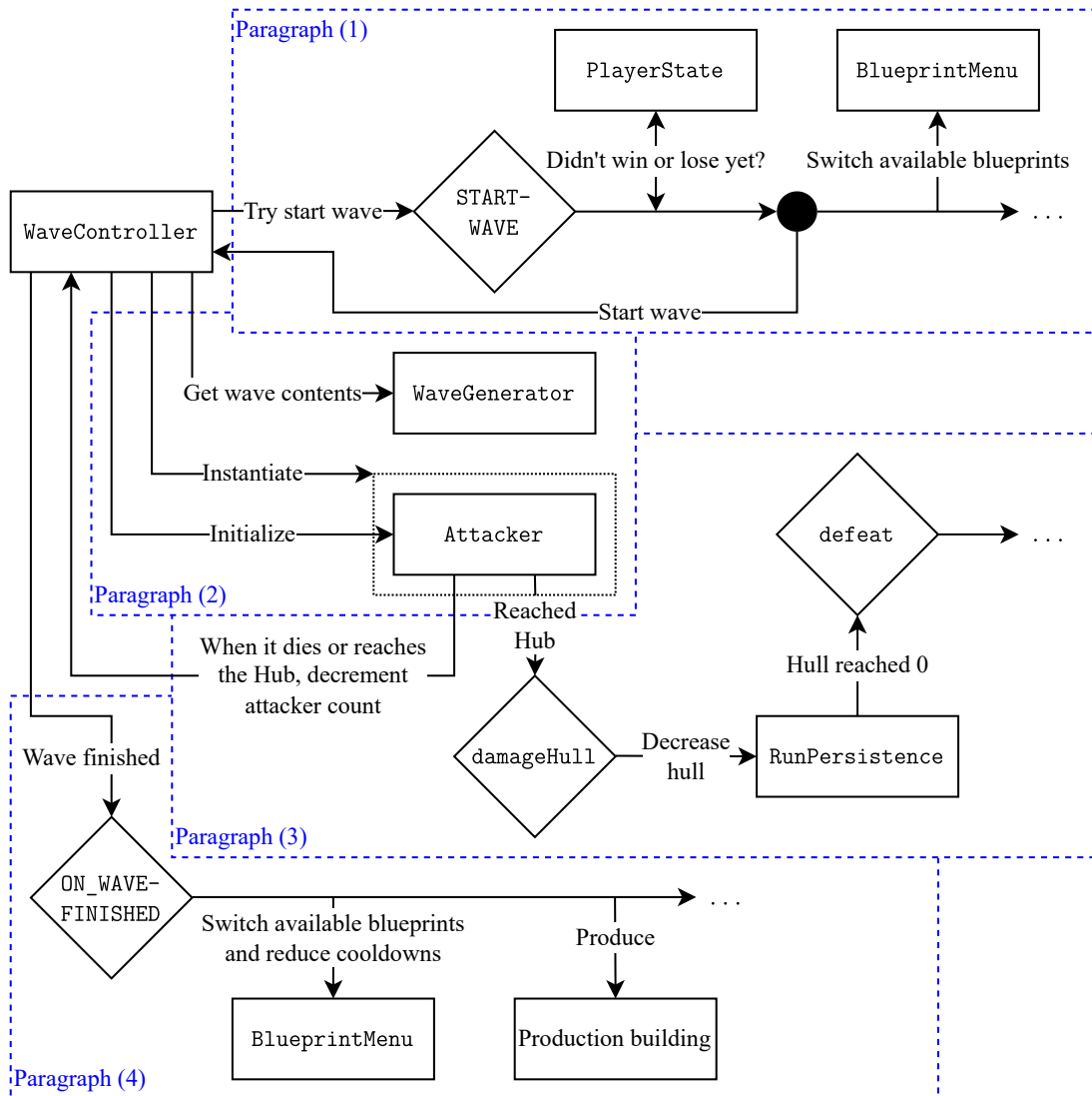
Figure 4.5 Interactions of WaveController with other scripts.
