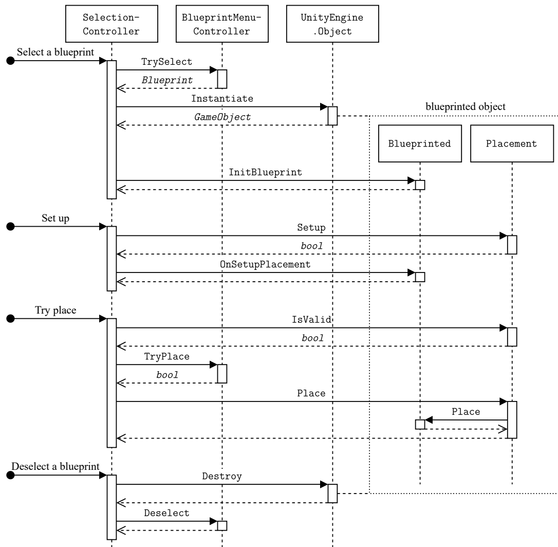
Figure 4.4 Sequence diagram of events related to placing a blueprint.
