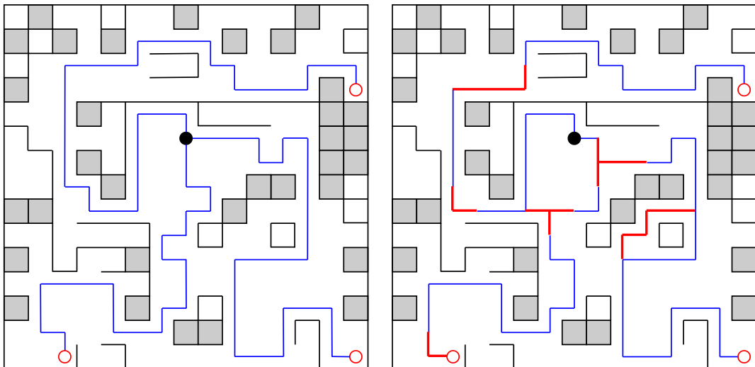
Figure 3.9 Final paths compared to the originally generated paths.
