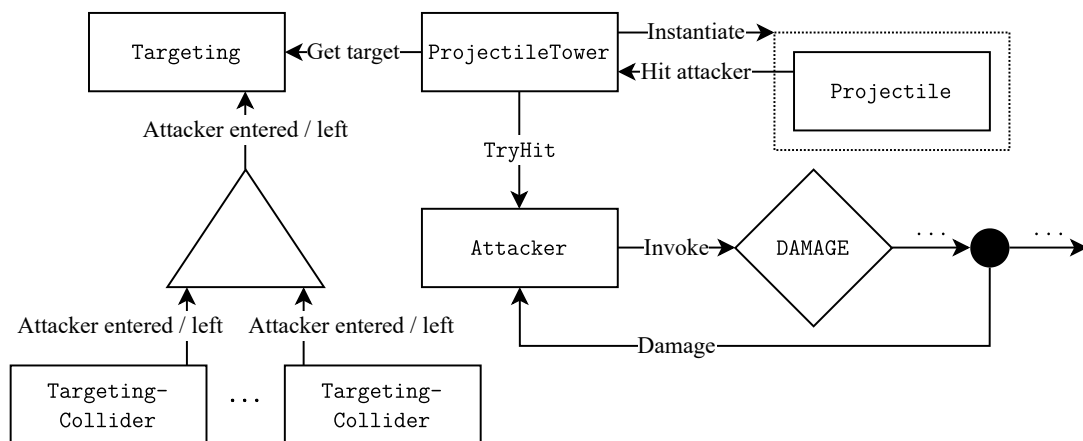
Figure 4.6 Script interactions when a tower shoots at an enemy.
