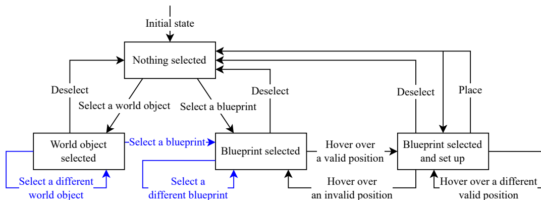
Figure 4.3 Selection states.
