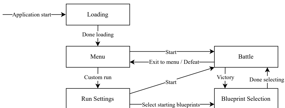
Figure 4.1 Scene transitions.
