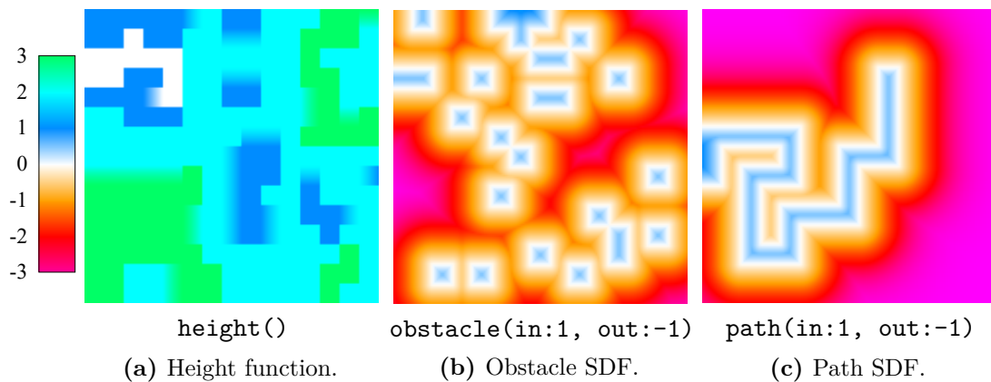
Figure 3.18 The values of the height function and signed distance functions.
