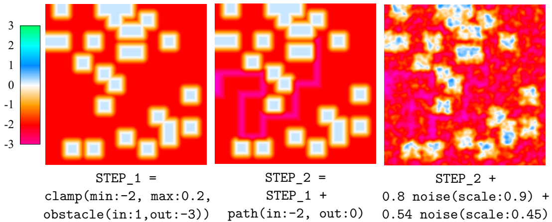
Figure 3.20 Building up a noise expression step by step.
