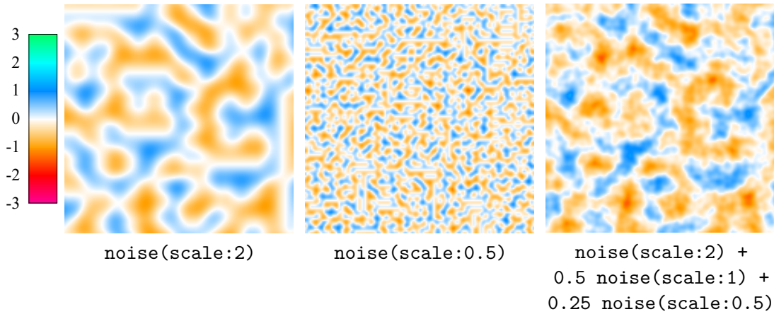
Figure 3.19 Examples of Perlin noise.
