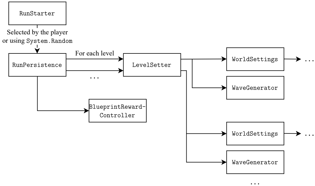
Figure 4.11 Seed propagation using seed branching.
