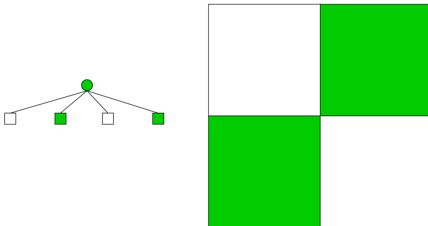
Figure 3.23 Quadtree range representation after expanding just the root node.
