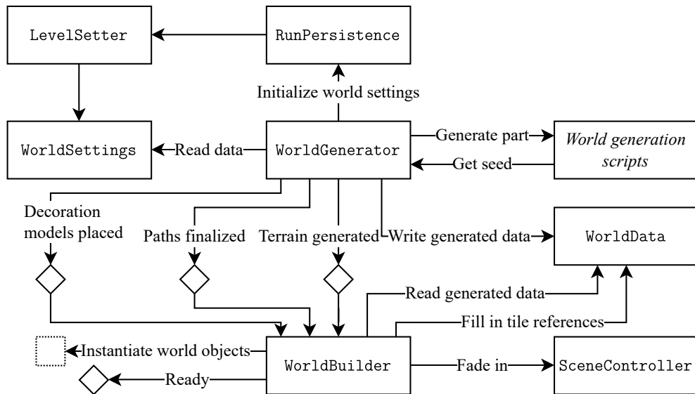
Figure 4.12 Script interactions during world generation.
