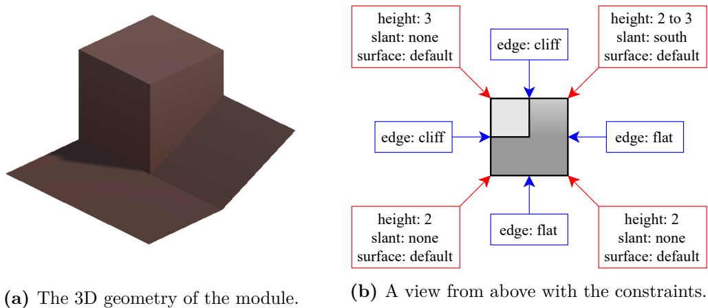
Figure 3.15 An example module and its constraints.
