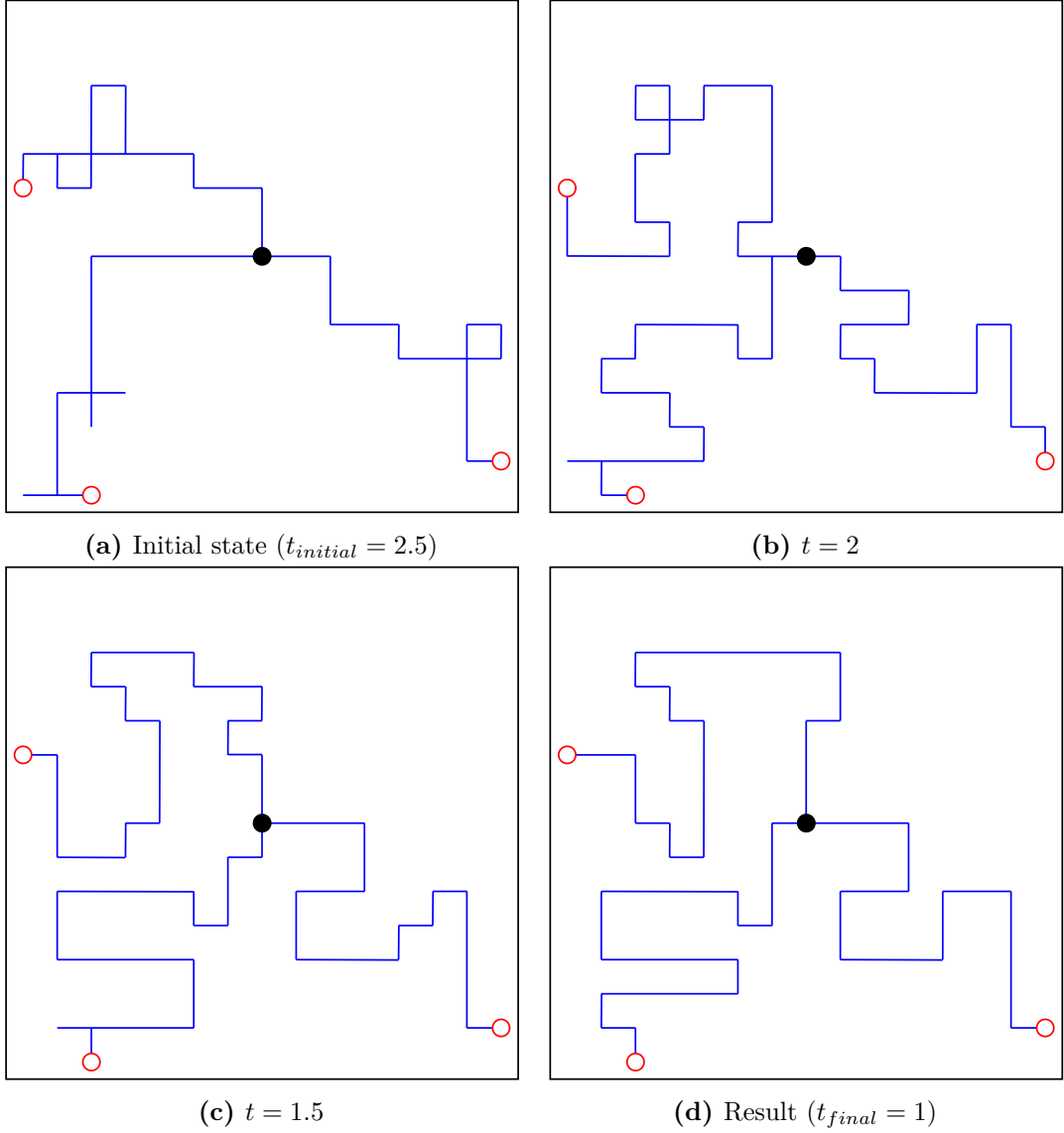
Figure 3.5 Evolution of paths during simulated annealing.
