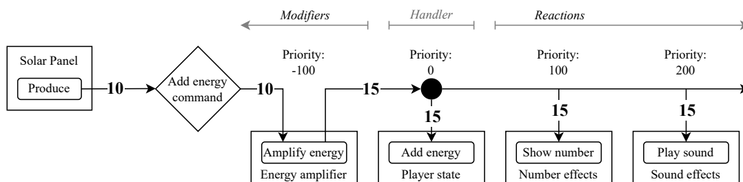
Figure 3.29 Modifiable command to add energy.
