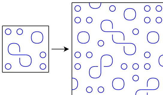
Figure 3.10 Example input and output of the wave function collapse algorithm.
