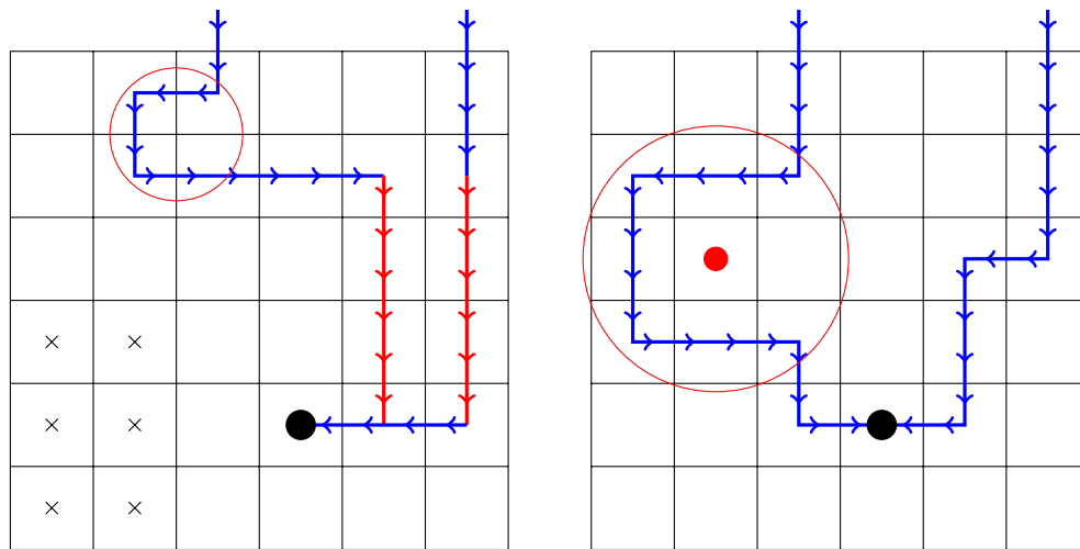
Figure 2.11 A path network with undesirable properties and a path network with great properties.
