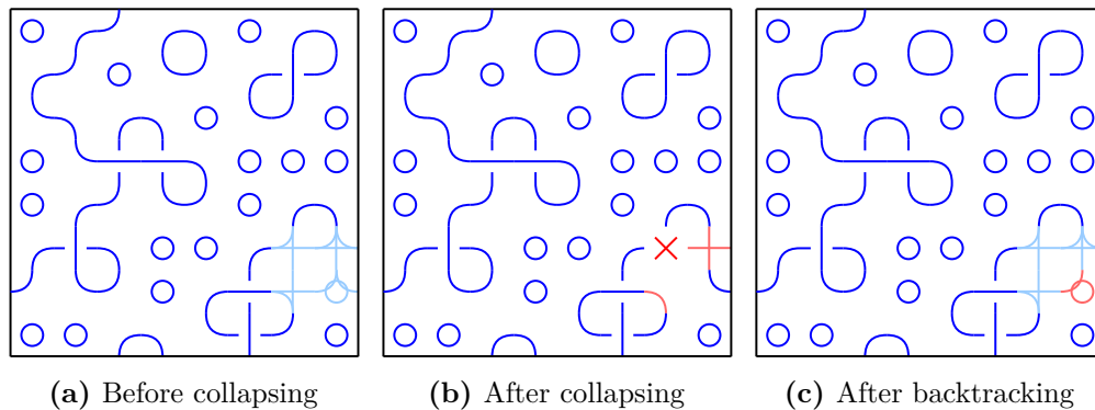
Figure 3.13 Conflicts and backtracking in WFC. The red cross marks a slot with no valid modules.
