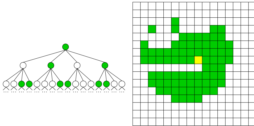
Figure 3.25 Quadtree range representation of a 16 \times 16 grid of sample points.
