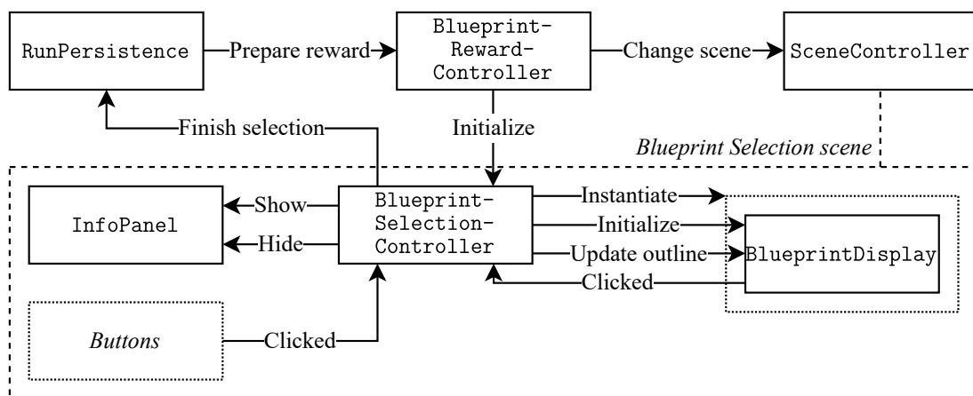
Figure 4.10 Interactions between scripts during blueprint selection.
