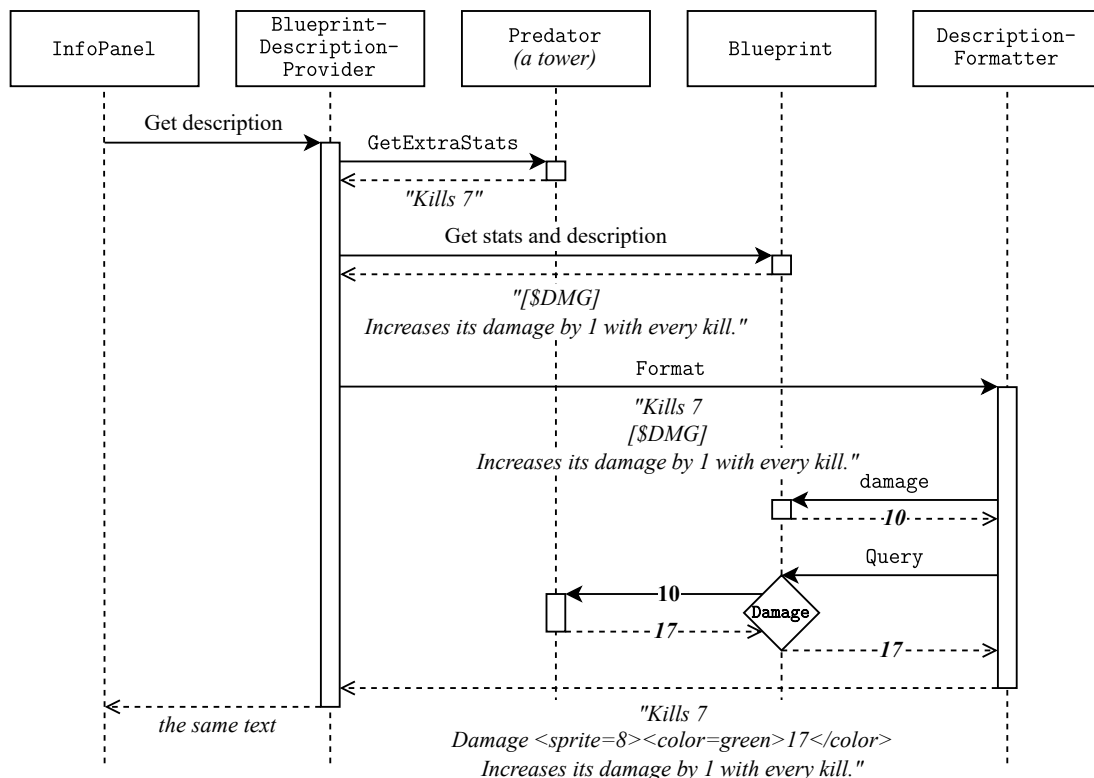
Figure 4.8 Generating the description to be shown in the info panel.
