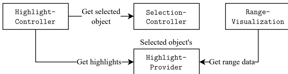
Figure 4.9 Interactions between scripts for highlights and range visualization.
