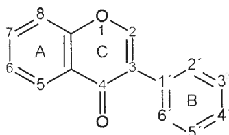
Figure 1-10 Flavanones.
